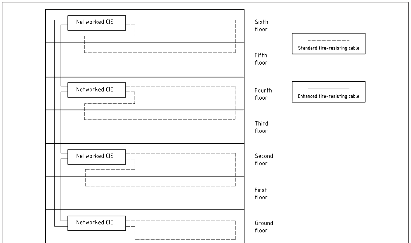
Figure 14 Example networked fire alarm systems (1 of 2)
