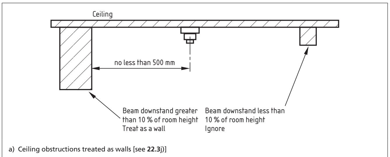
Figure 10 Ceilings (1 of 2)
