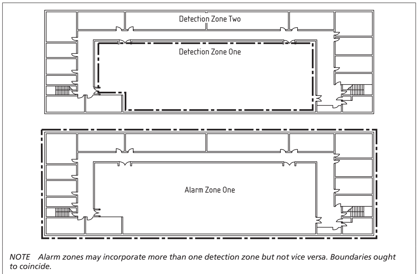
Figure 3 Alarm zones [see 14.2d)]
