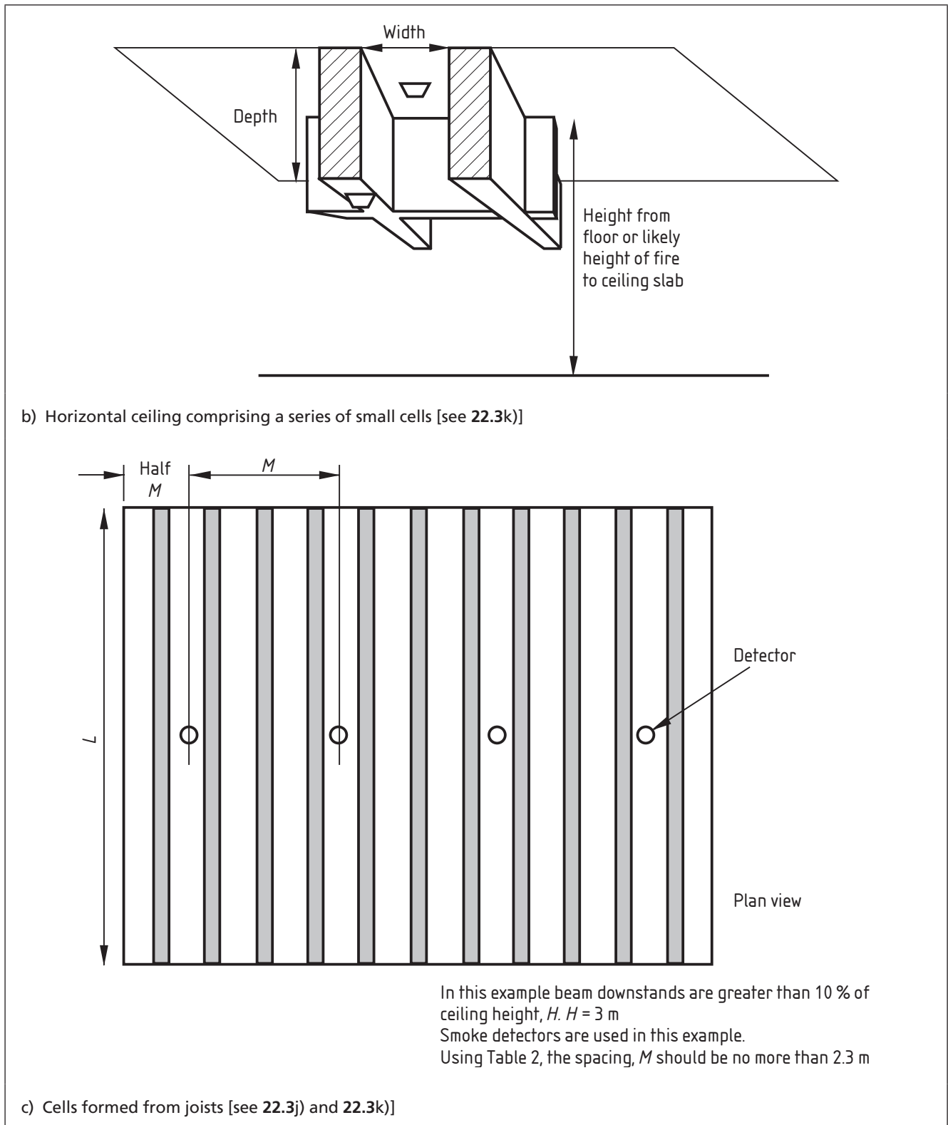
Figure 10 Ceilings (2 of 2)
