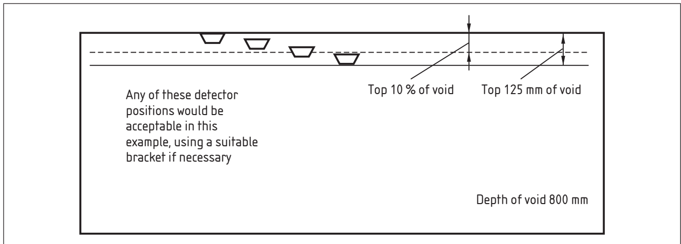
Figure 7 Detectors in top 10% of a void [see 22.3f)]
